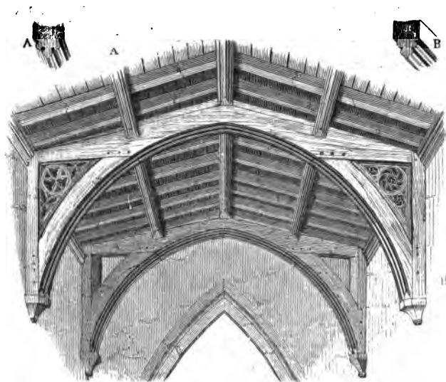
136. Sparsholt, Berkshire, c. 1350.
